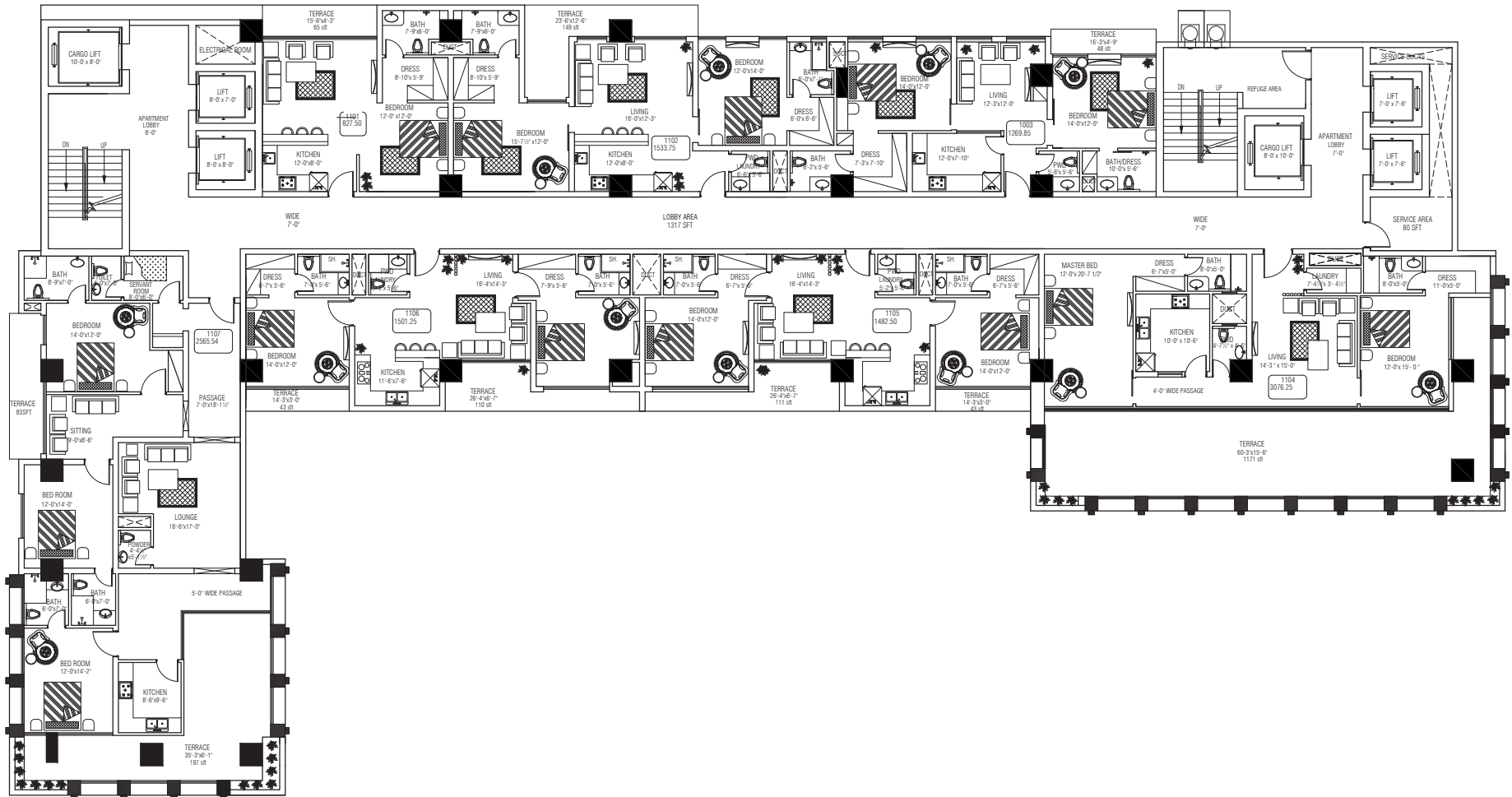
ELEVENTH FLOOR PLAN
